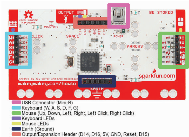
Gambar 9-3 Bagian Belakang Papan Sirkuit Makey Makey Sumber: https://content.instructables.com/ORIG/FTH/AZRK/HTSYZXO9/FTHAZRKHTSYZXO9.jpg?auto=webp&frame=1&it=bounds&md=d07d1c5d975da3b0839e268280e23aa6
