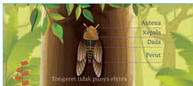
Gambar 5. Anatomi tonggeret
